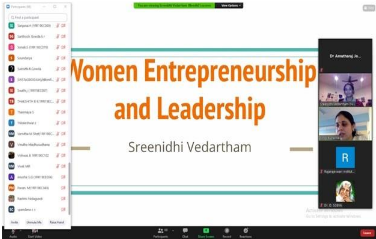
Sample Screenshots
