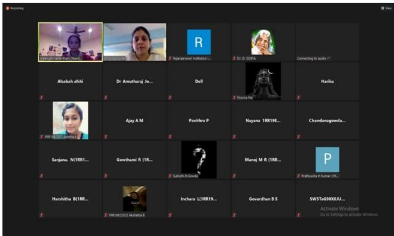
Sample Screenshots
